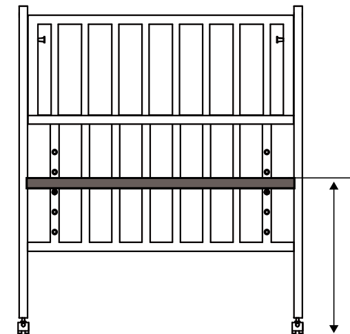
床板高さH=48cm
